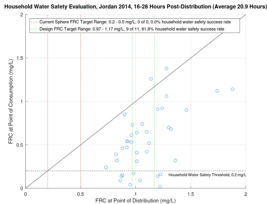
Fig. 7. Household water safety evaluation of site-specific FRC target compared to Sphere FRC target, Jordan 2014; data included from samples with household follow-up at 16-28 hours post-distribution (average 20.9 hours).
