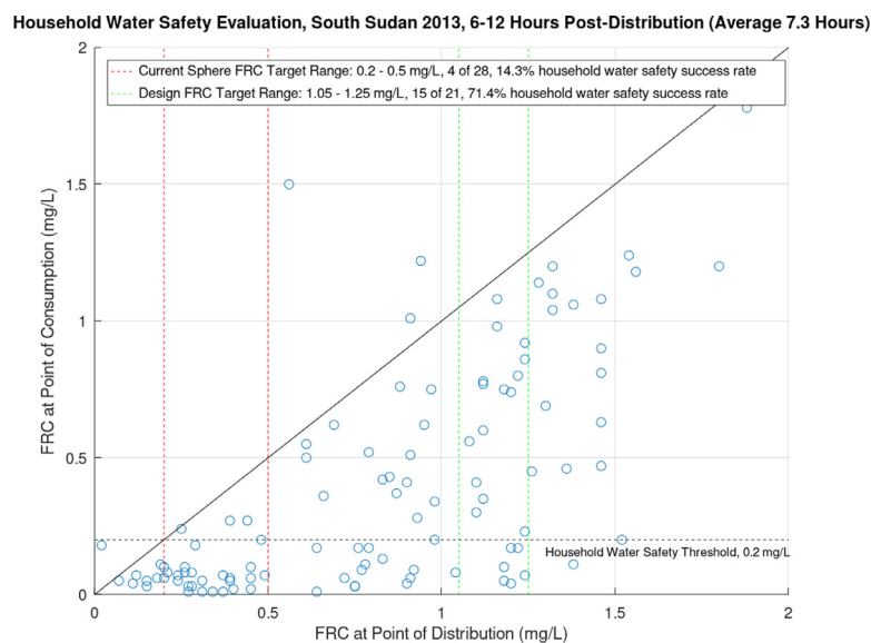
Fig. 5. Household water safety evaluation of site-specific FRC target compared to Sphere FRC target, South Sudan 2013; data included from samples with household follow-up at 6-12 hours post-distribution (average 7.3 hours).
